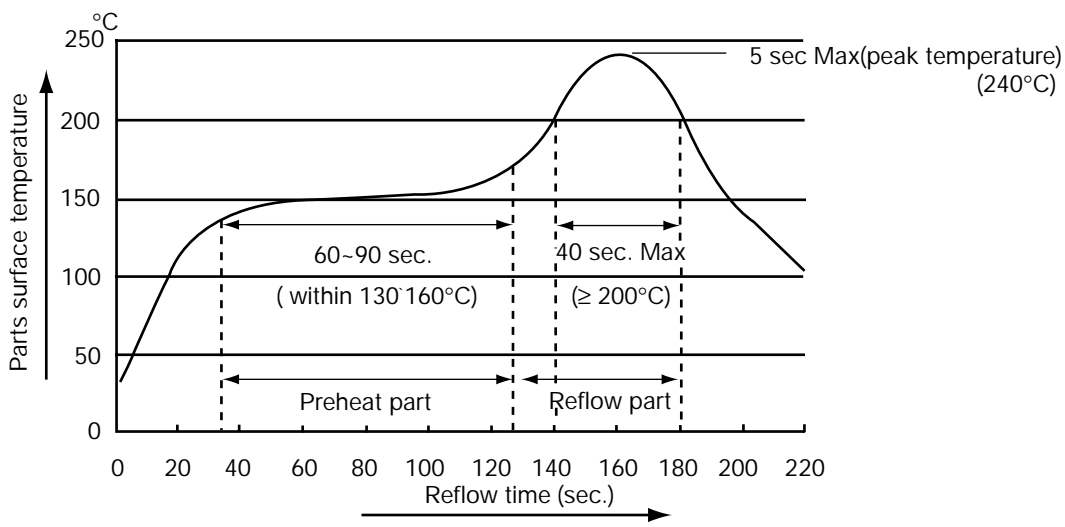
Soldering Temperature Profile (Reflowing soldering)
