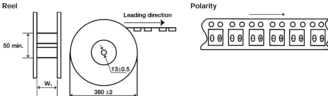
Tape and Reel Specifications
